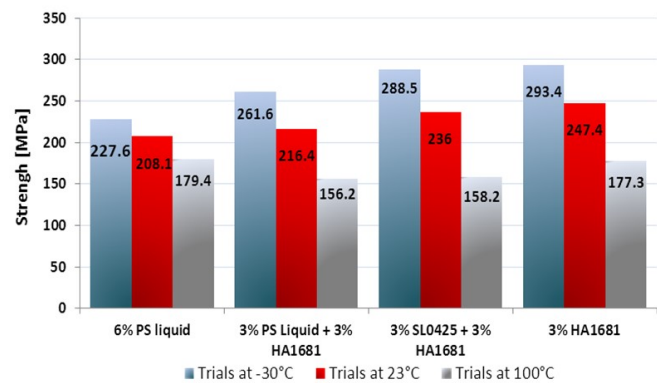
Maximum strength - Impact Multi axis
