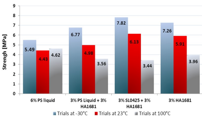
Flexural strength - Impact Multi axis
